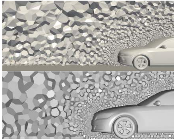
Figure 15: Comparison of rendering obtained from ParaView (first picture) and ViZiR 4 (second picture). In the first case, shading is done by triangle while it is done by polygon in the second case.
