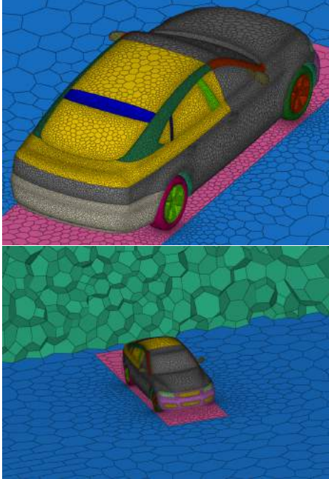
Figure 1: Examples of meshes composed of polygons only (top) and polygons and polyhedra (bottom). The number of vertices is not constant by element.
