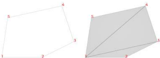
Figure 6: A 5-sided convex polygon. The naive tessellation algorithm 1 works.
