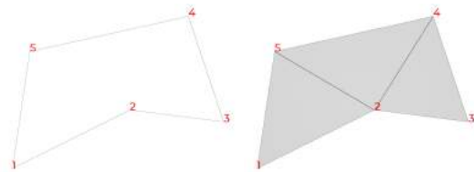
Figure 8: A 5-sided concave polygon. Following algorithm 2, a concave vertex (here vertex 2) has been used as a starting point to create the tessellation.
