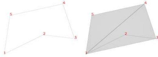
Figure 7: A 5-sided concave polygon. The naive tessellation algorithm 1 fails.
