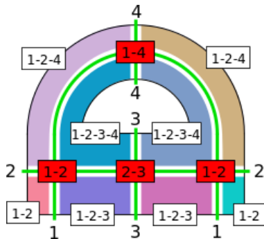
Figure 16: As two dual lines can intersect each other more that once, dual node and dual zone labeling is not unique.
